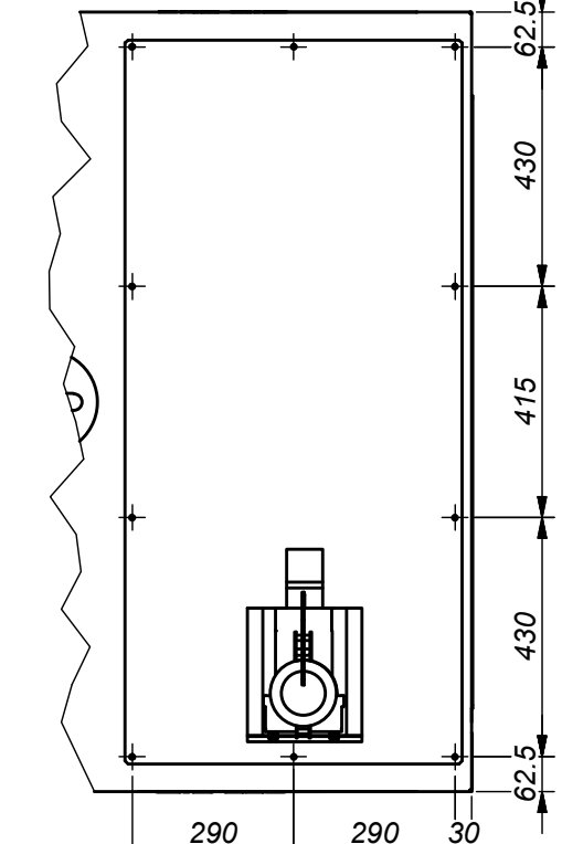
( FRONT OUTLET ) ( 1 : 15 )
