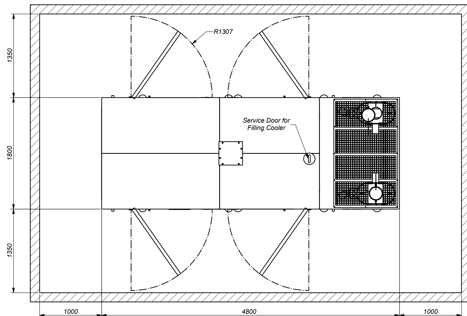
MAINTENANCE SPACE (1:30)
